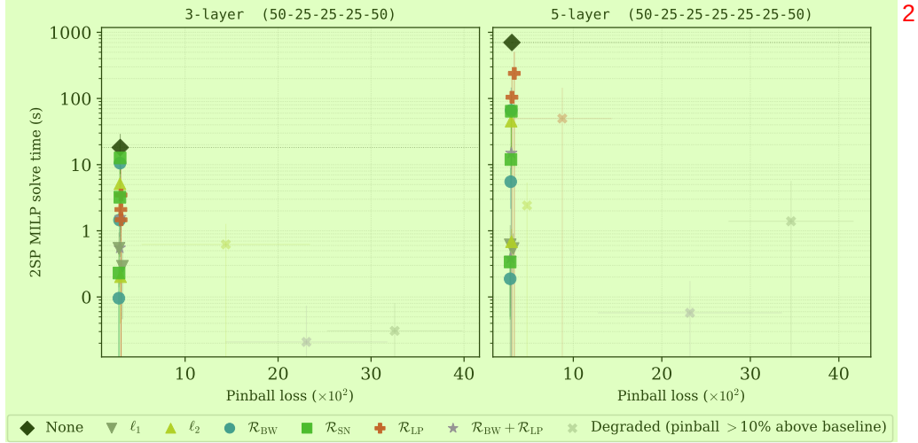
Fig. 5 Tradeoff between solution time of downstream MILP performance and pinball loss for QNNs in stochastic programming setting. Each plotted marker shows mean performance for a different regularizer and weight.
