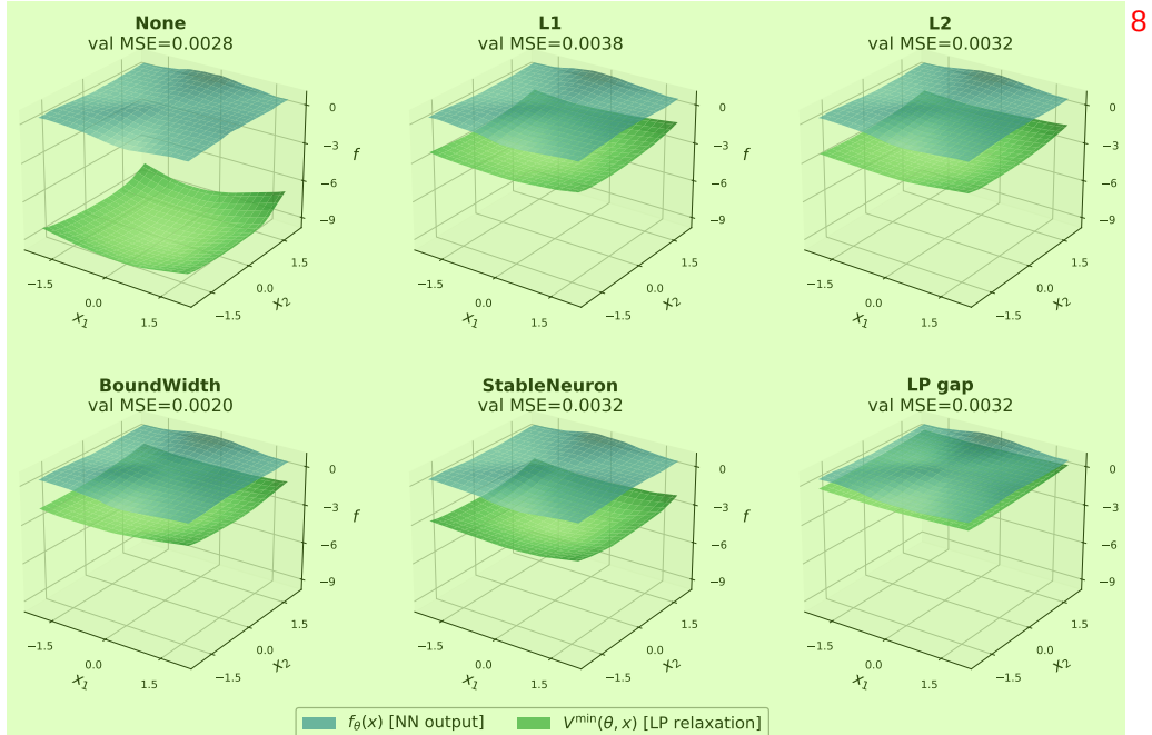
Fig. 1 Predictions and LP lower bounds for NN models with \{32, 32\} hidden layers trained on the scaled Peaks function with two inputs (x_1, x_2) , with output f(x) . Different regularizers are applied during training, with weights chosen to maintain validation MSE of similar scale.
