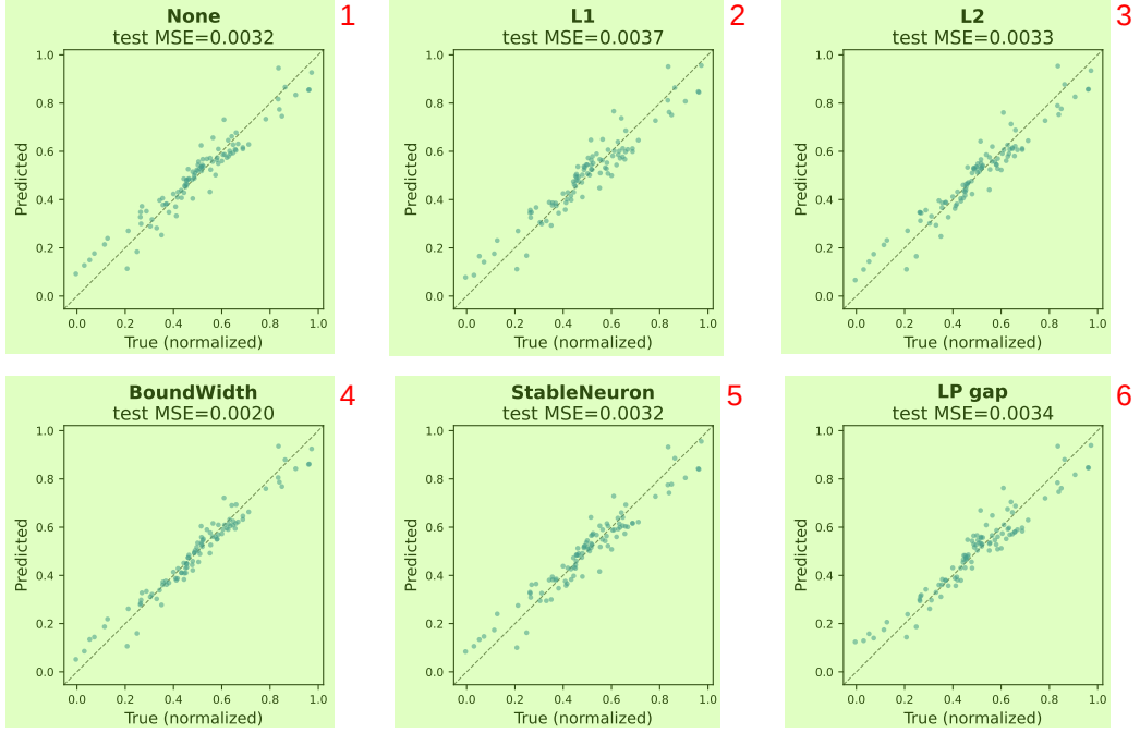
Fig. 4 Parity plots for NN models with \{32,32\} hidden layers trained on the scaled Peaks function with two inputs (x_1, x_2) , with output f(x) . Different regularizers are applied during training, with weights chosen to maintain validation MSE of similar scale. 7
